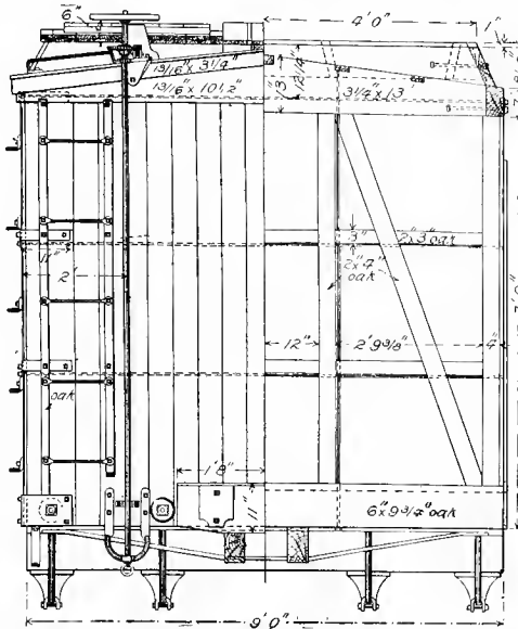
Fig. 276. End Elevation.
